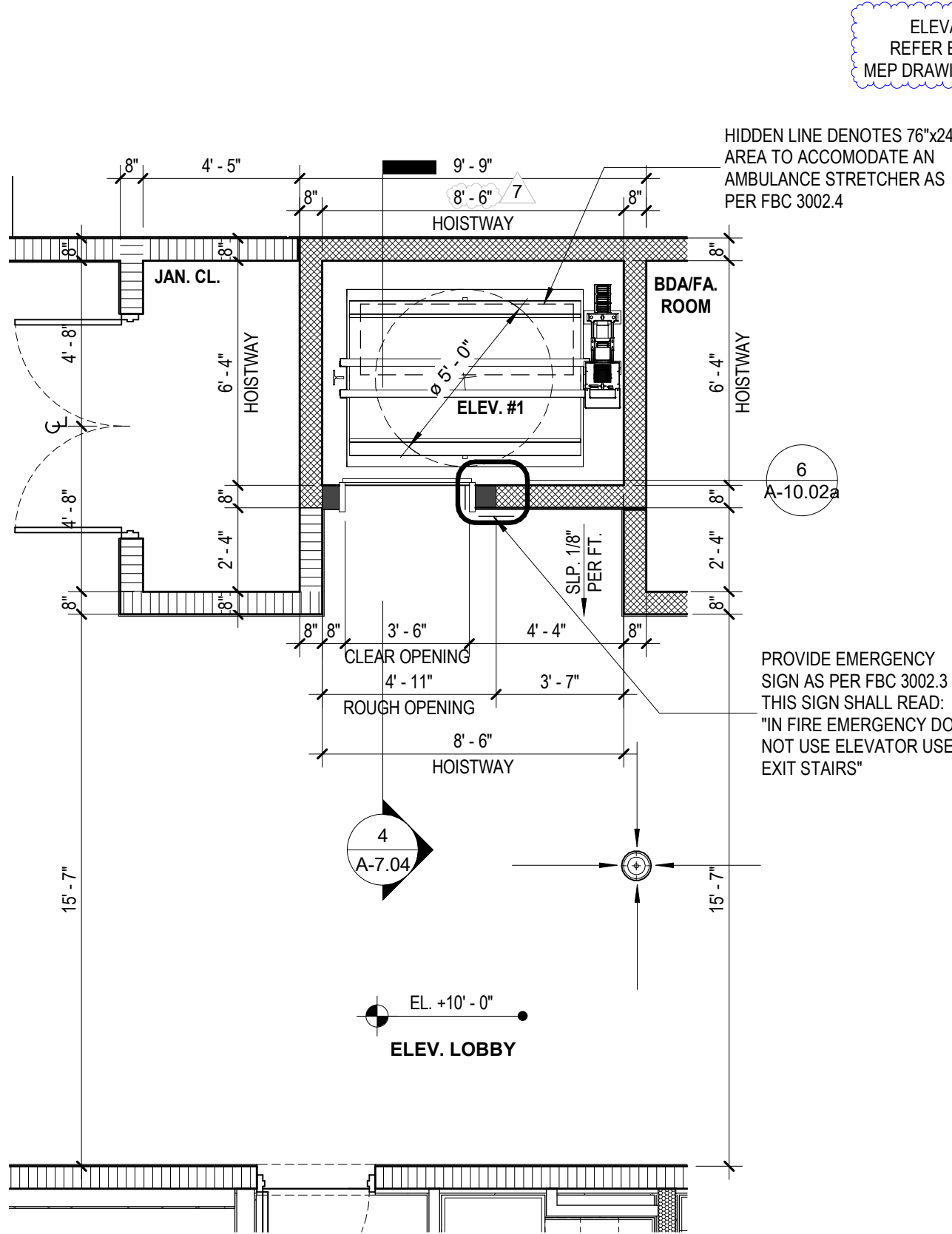
1 BLDG A - ELEV. @ GROUND FLOOR SCALE: 1/4" = 1'-0"
