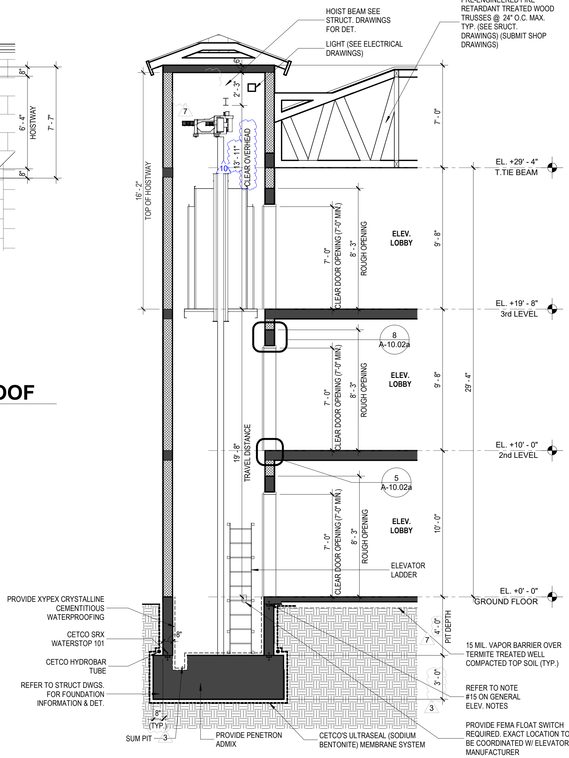
4 BLDG A ELEV. SECTION SCALE: 1/4" = 1'-0"
